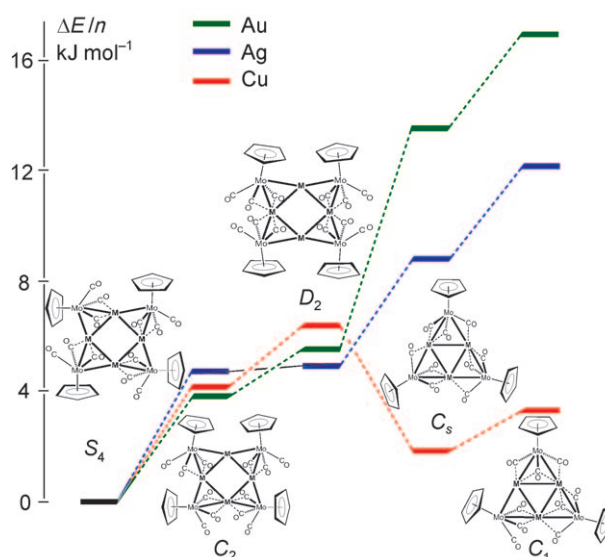
Figure 4. Representation of the relative energies computed for various possible structures of [M\{MoCp(CO)_3\}]_n ( M = Cu, Ag, Au; n = 3, 4 ) and reduced to a single hypothetical monomer ( n = 1 ). For each metal M , the zero-energy level of the monomer corresponds to the square structure of S_4 symmetry.
